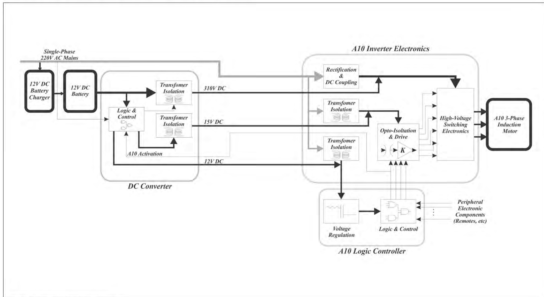
Fig. 4 DC Converter and A10 Schematic Diagram
